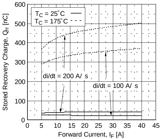
Figure 23. Stored Charge
