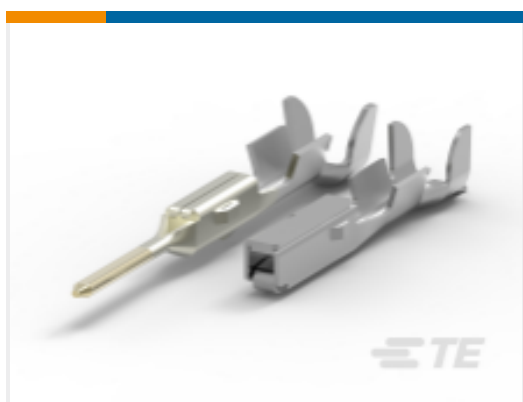
TE Part #1897598-1 MULTILOCK, RECEPTACLE AND TAB
