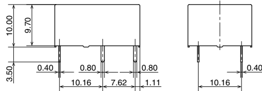
2 coil latching type
