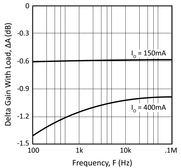
Figure 18: Loading Effects
