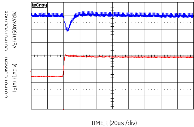
Figure 28. Transient Response to Dynamic Load Change from 50% to 100% at 12Vin, Cout-2x47uF, CTune-2200pF & RTune-261
