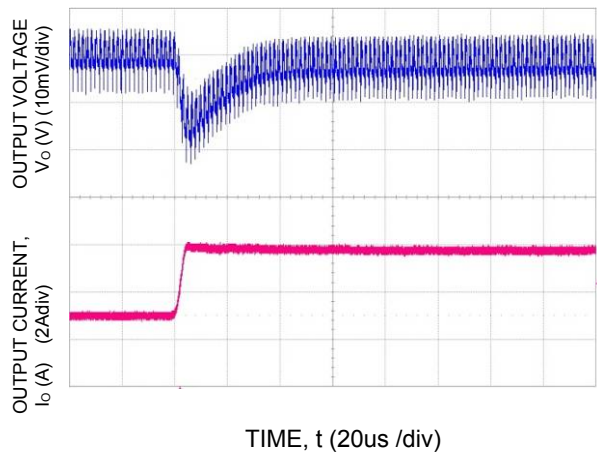
Figure 42. Transient Response to Dynamic Load Change from 50% to 100% at 12Vin, Cout=1x47uF + 2x330uF, CTune=12nF, RTune=178
