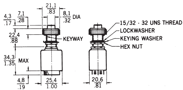
Watertight Switch
