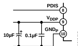
Figure 16. V_{DDP} Bias and Bypass Components
