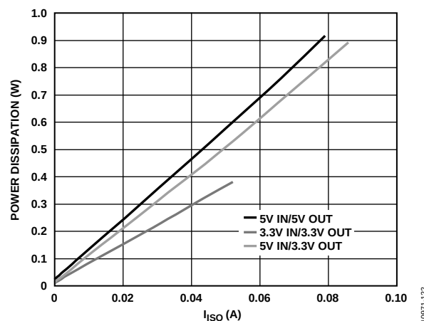
Figure 6. Typical Total Power Dissipation vs. Isolated Output Supply Current in All Supported Power Configurations
