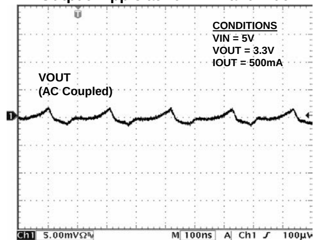
Output Ripple at 20MHz Bandwidth
