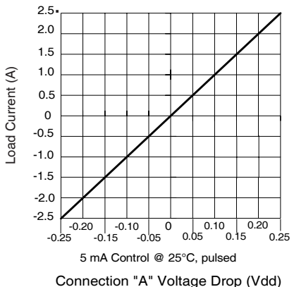
Figure 3. Linearity Characteristics
