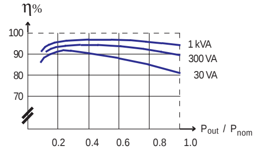
Graph 4 (Efficiency)
