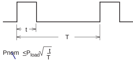
Graph 3 (Duty Cycle)
