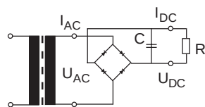
Graph 7 (Rectifying)
