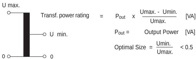
Graph 1 (Autotransformers)
