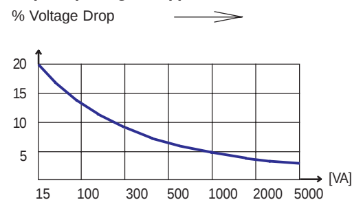
Graph 2 (Voltage Drop)
